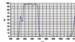
Transmission Fringe-Killer Filter
